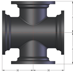
MJ Cross
