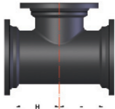
MJ Tee
