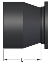
MJ Small End Reducer SEB
