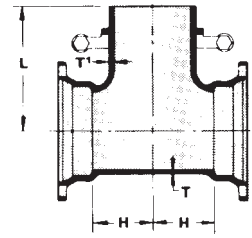
Hydrant Tee
